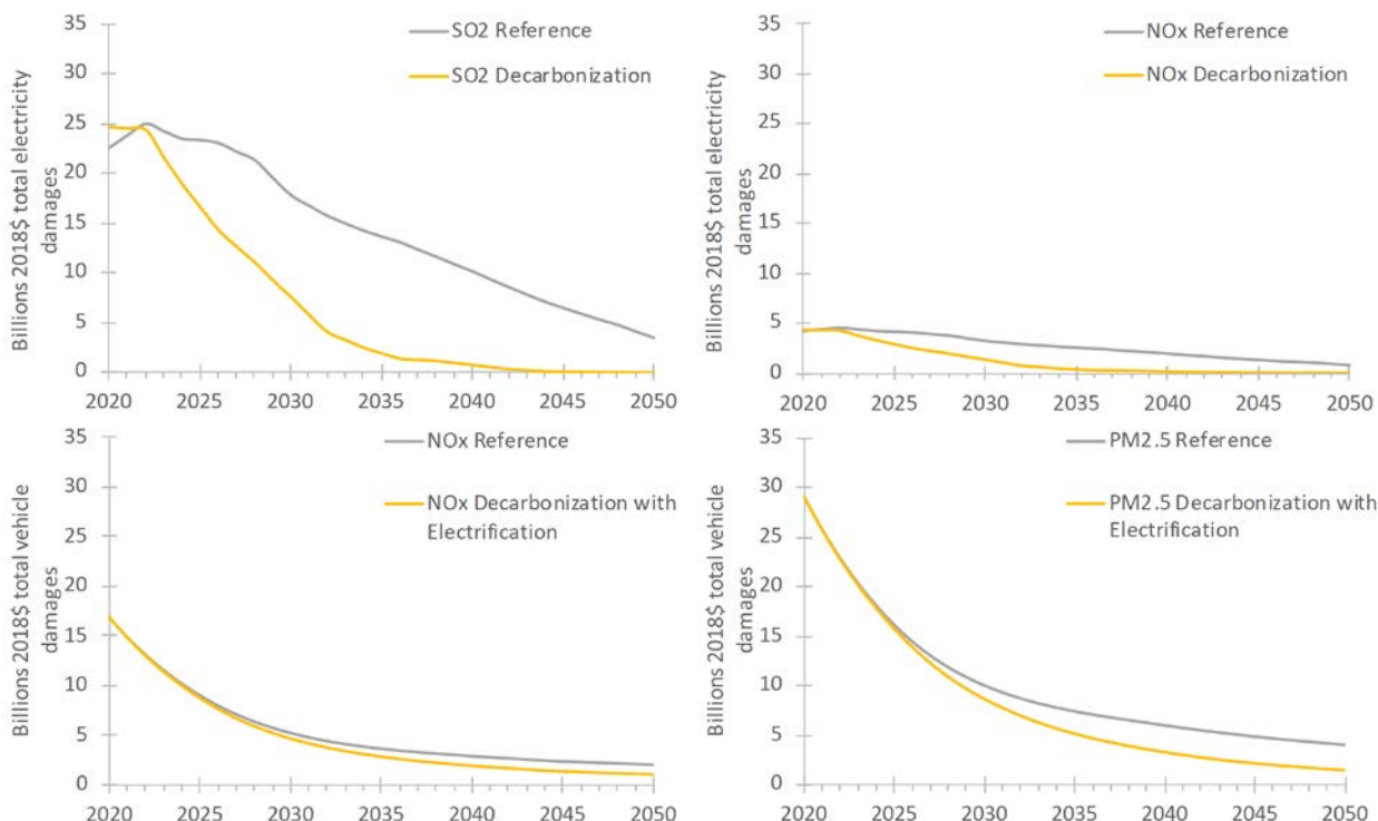
Figure C-8. Discounted annual damages by sector, pollutant, and scenario
