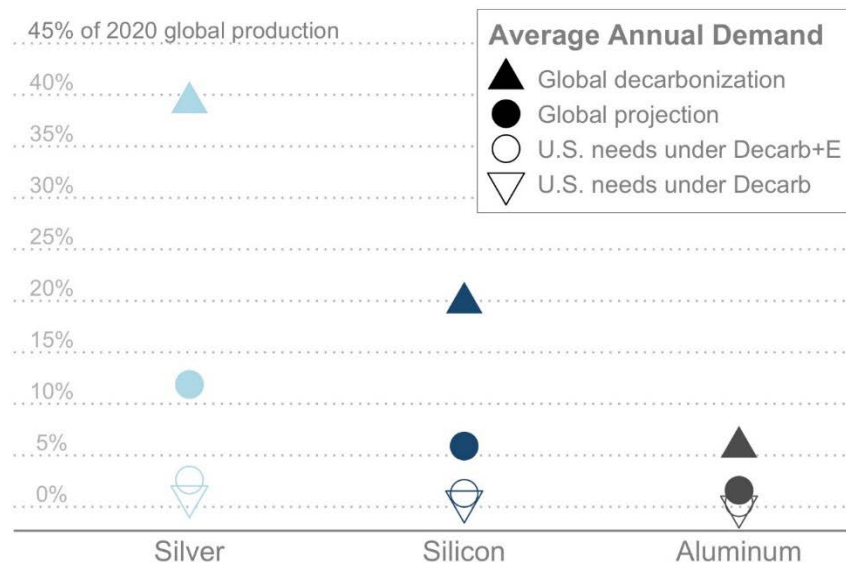
Figure 7. Percentage of 2020 global production of various materials needed to supply average annual virgin materials demand for c-Si PV in the two decarbonization-based Solar Futures Study scenarios
