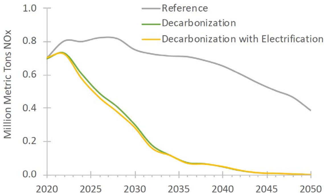
Figure 15. Total NO x emissions from the power sector in the Solar Futures Study core scenarios
