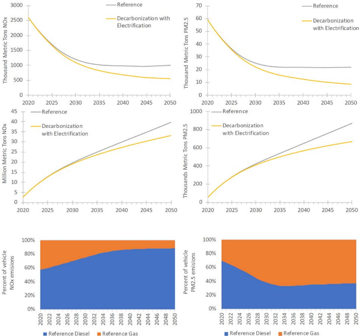
Figure C-5. Total annual (top) and cumulative (middle) NO x and PM 2.5 emissions from vehicles and (bottom) split of emissions by diesel or gasoline vehicles within the Reference scenario
