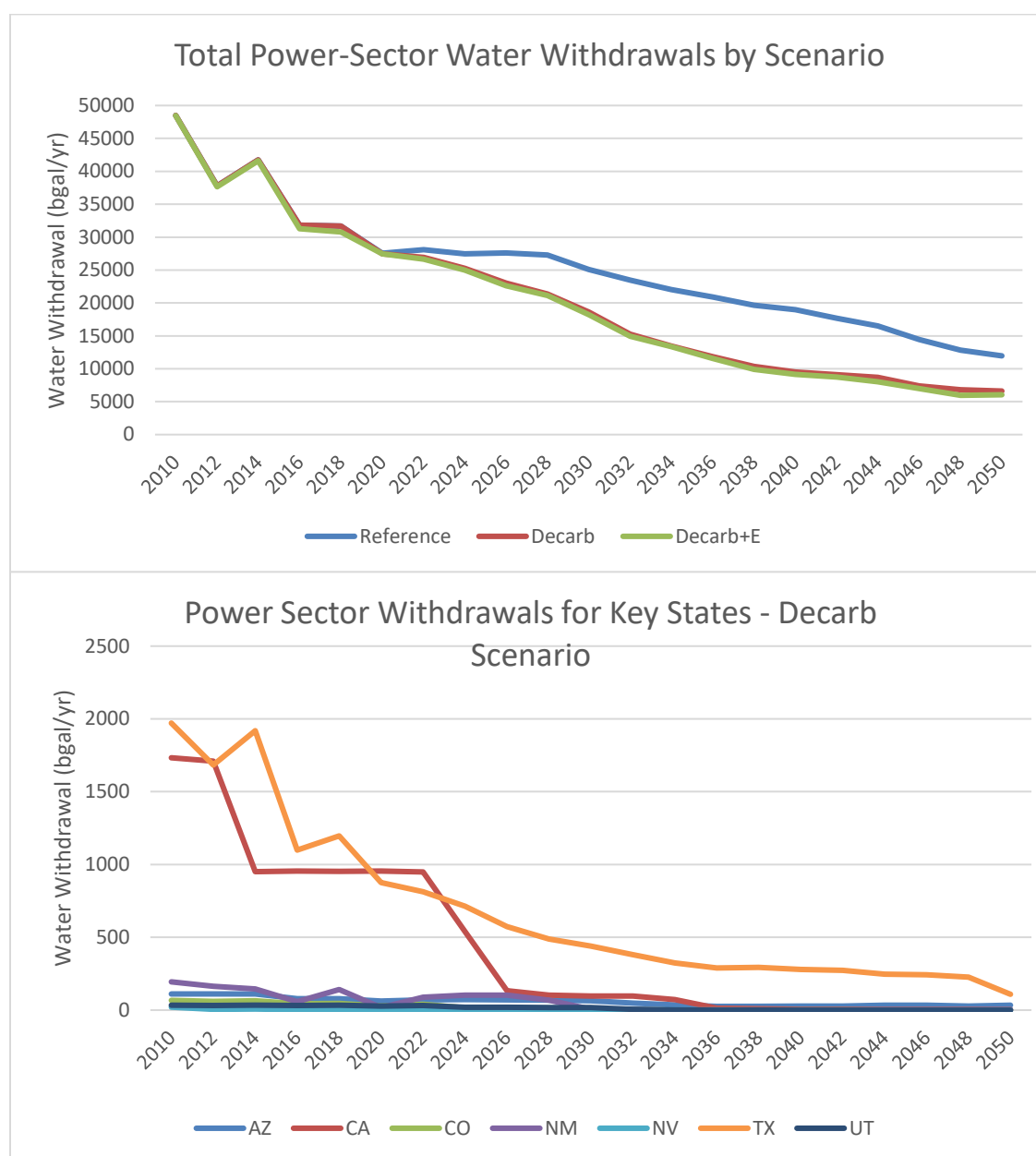
Figure 11. Total U.S. power-sector water withdrawals under the Solar Futures Study core scenarios (top) and withdrawals for key states in the Decarb scenario (bottom), assuming water constraints
