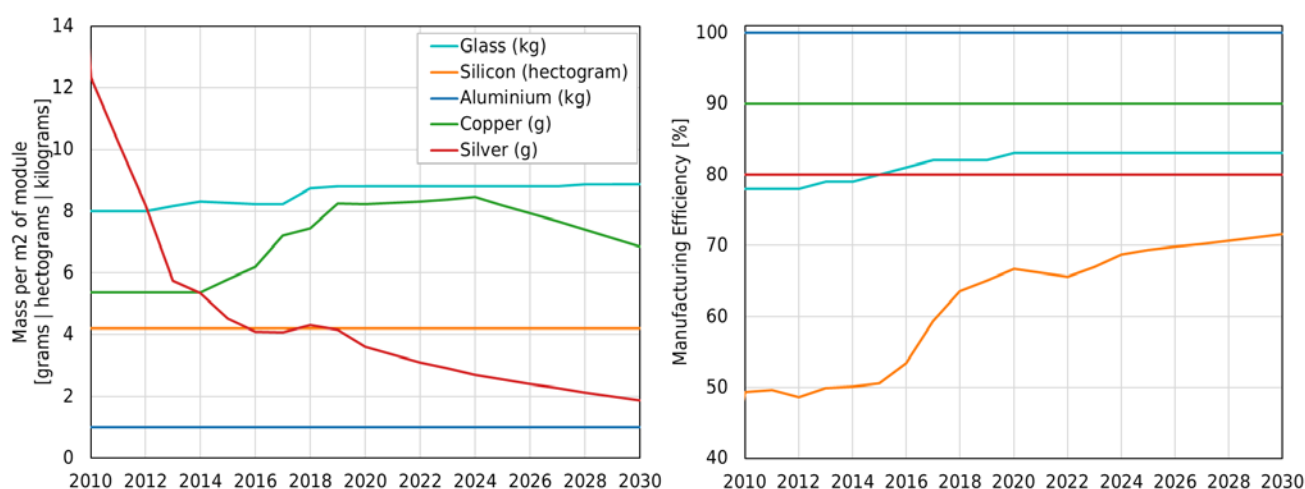
Figure B-2. All materials on a mass per meter squared of module basis over time (a) and the manufacturing efficiency of all materials over time (b)
