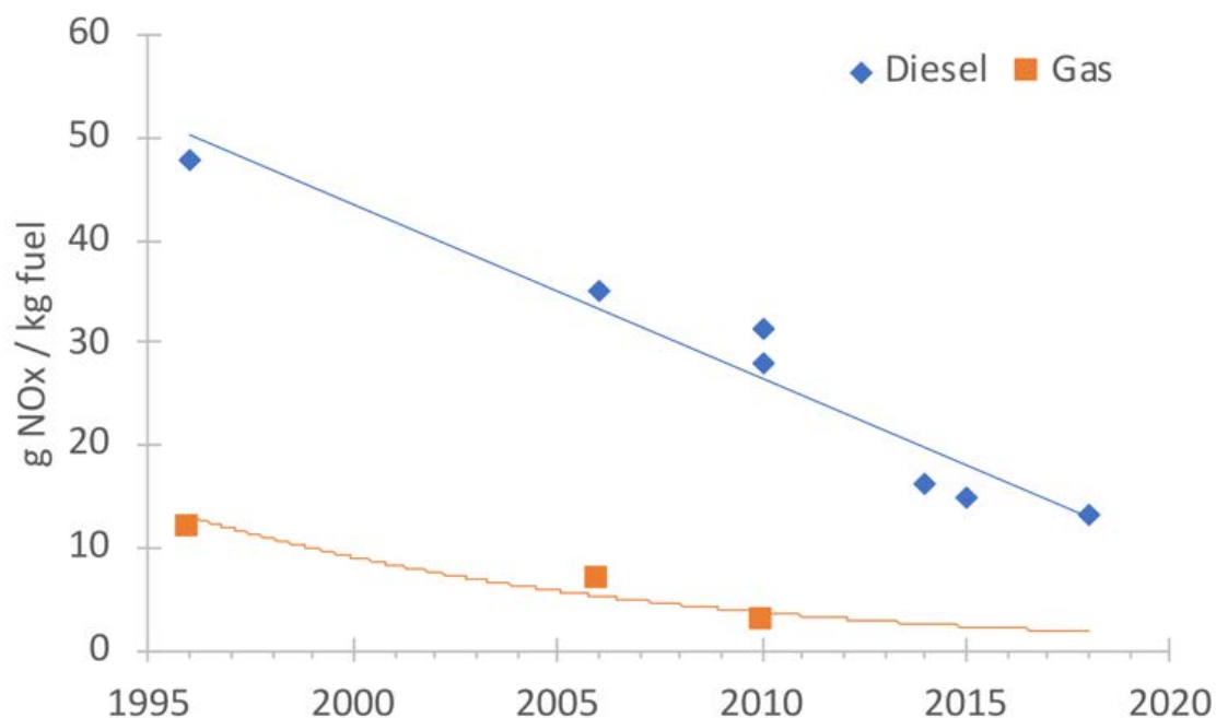
Figure 16. Fleet-average NO x emission rates of U.S. light-duty gasoline vehicles and heavy-duty diesel trucks, based on observed emissions 194–197
