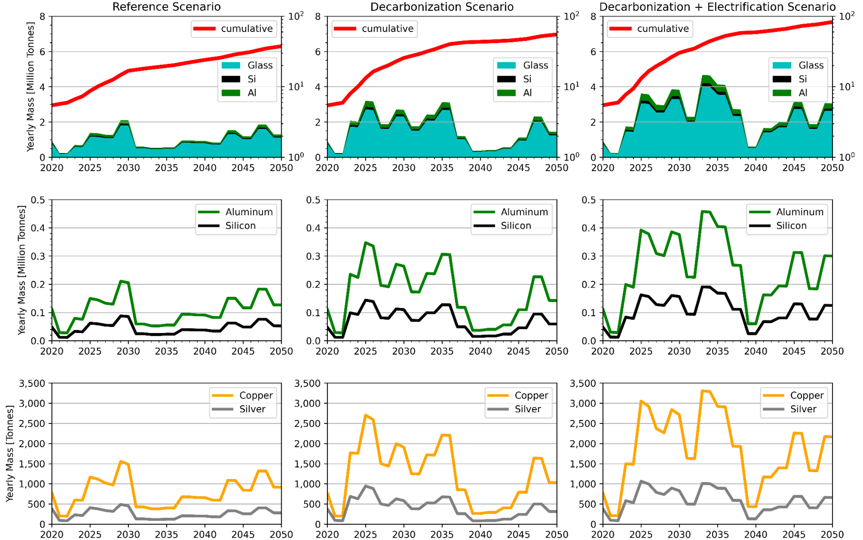
Figure 6. Annual demand of selected materials for PV manufacturing across the three core Solar Futures scenarios, 2020–2050
