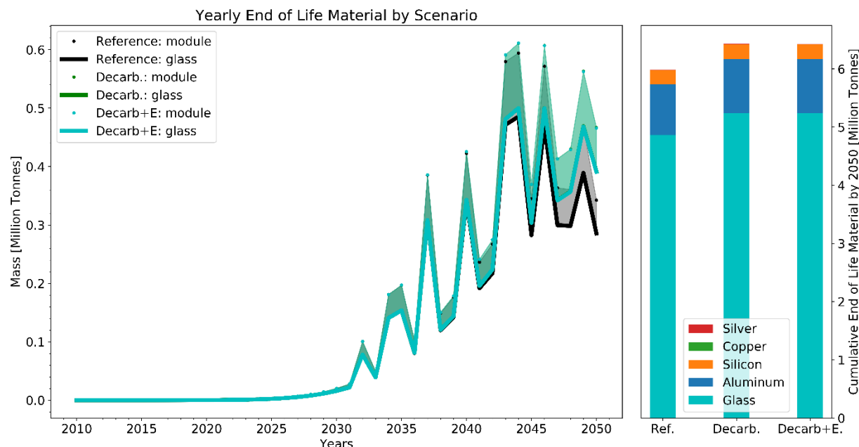
Figure 19. Annual and cumulative PV EOL material mass by Solar Futures Study scenario through 2050
