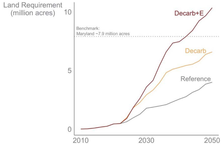
Figure 9. National solar land-use projections for the three core scenarios, 2010–2050
