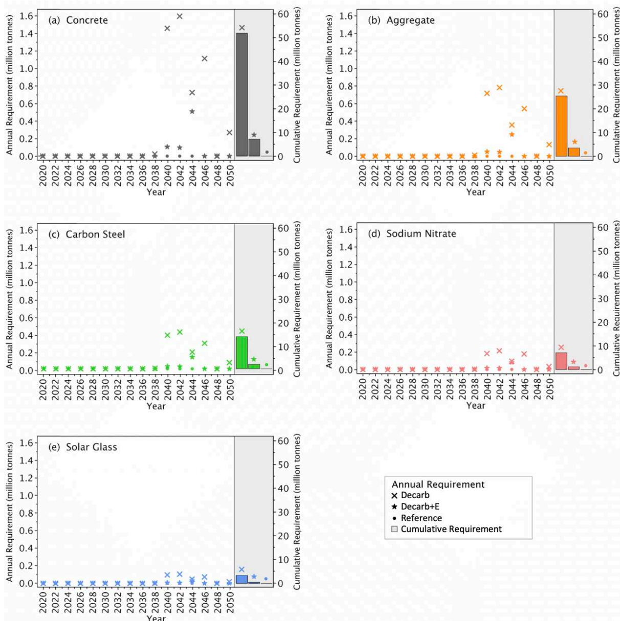
Figure 8. Five most-used materials in the manufacturing and construction of power tower CSP plants in the three core Solar Futures Study scenarios
