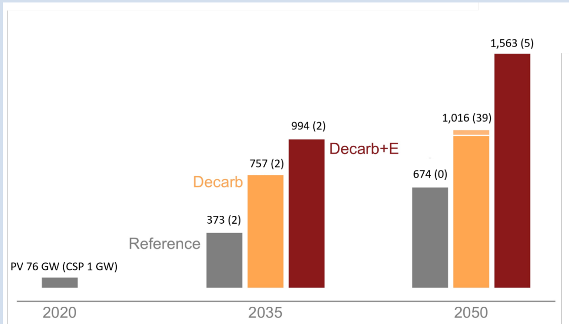
Figure 2. Cumulative deployed capacity of PV and CSP in 2020, 2030, and 2050 in the three core Solar Futures scenarios
