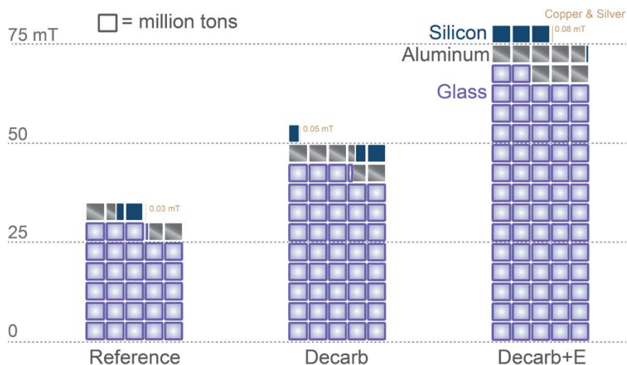
Figure 5. Comparison of virgin material demands for each silicon-based PV material cumulatively (2020–2050) across the three scenarios
