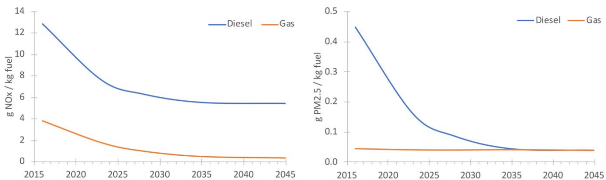
Figure C-4. Future vehicle NO x and PM 2.5 emission rates based on EPA MOVES model
