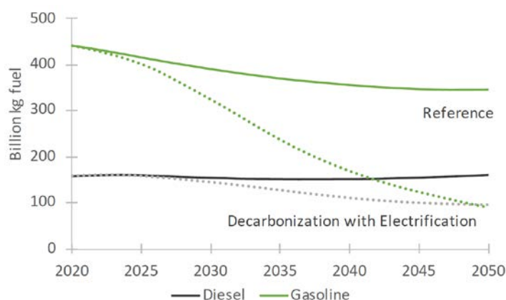
Figure C-2. Total vehicle fuel use by scenario
