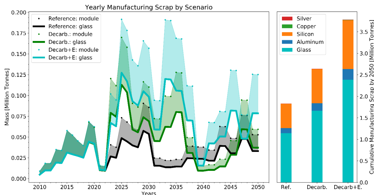
Figure 20. Annual and cumulative mass of c-Si PV manufacturing scrap by Solar Futures Study scenario through 2050
