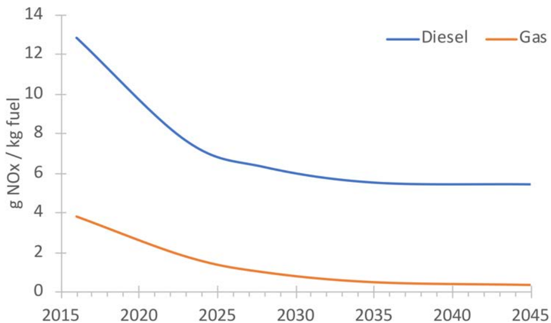
Figure 17. Future fleet-average NO x emission rates for U.S. light-duty gasoline vehicles and heavy-duty diesel trucks based on the EPA MOVES model
