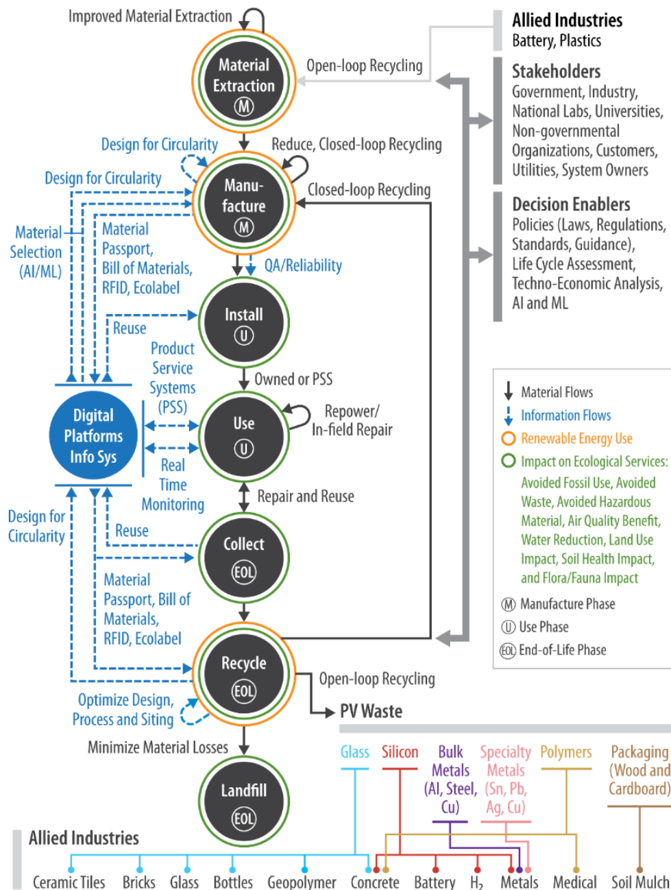
Figure 3. Systems framework to assess the current state-of-the-art and identify opportunities to advance the CE for PV
