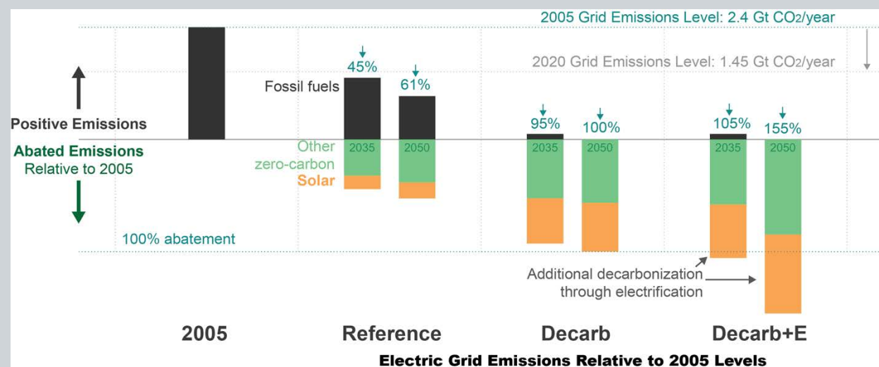
Figure 1. Grid emissions and abated grid emissions by Solar Futures scenario in 2035 and 2050, relative to 2005 grid emissions 1
