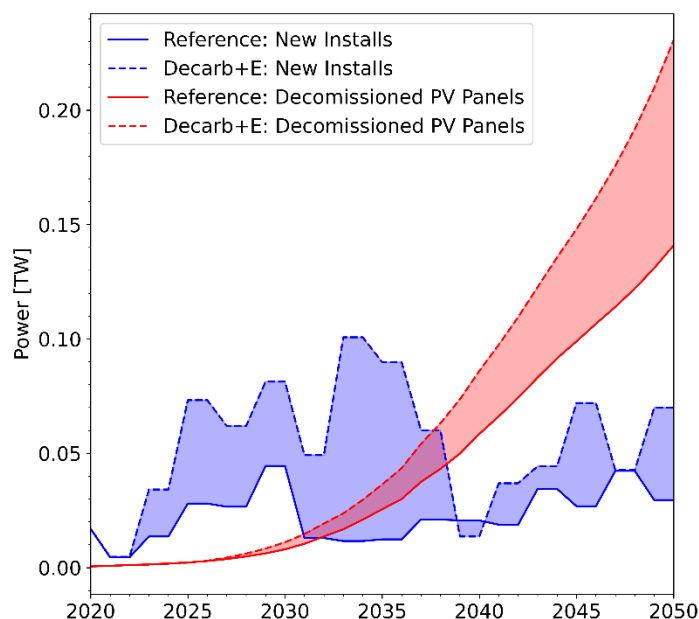
Figure 22. Annual installations and decommissions for 2020 through 2050
