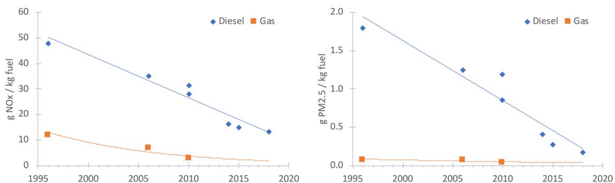
Figure C-3. Fleet-average NO x and PM 2.5 emission rates of light-duty cars and heavy-duty diesel trucks, based on observed emissions 194–197
