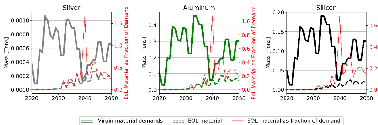
Figure 23. Yearly virgin material demands and EOL silver, aluminum, and silicon, with right axis showing the fraction of Decarb+E scenario demand that could be supplied by the EOL material
